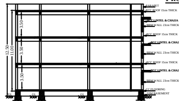
SECTIONAL ELEVATION
